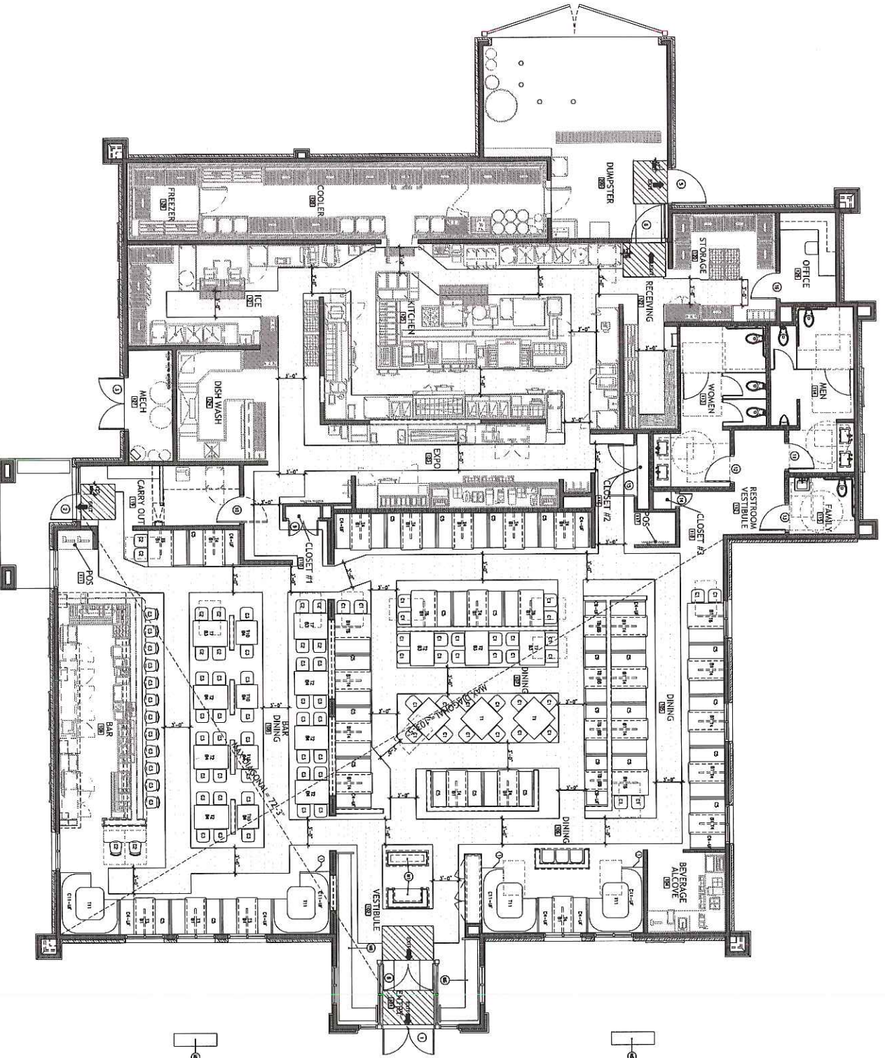
FURNISHING/EGRESS FLOOR PLAN 1
