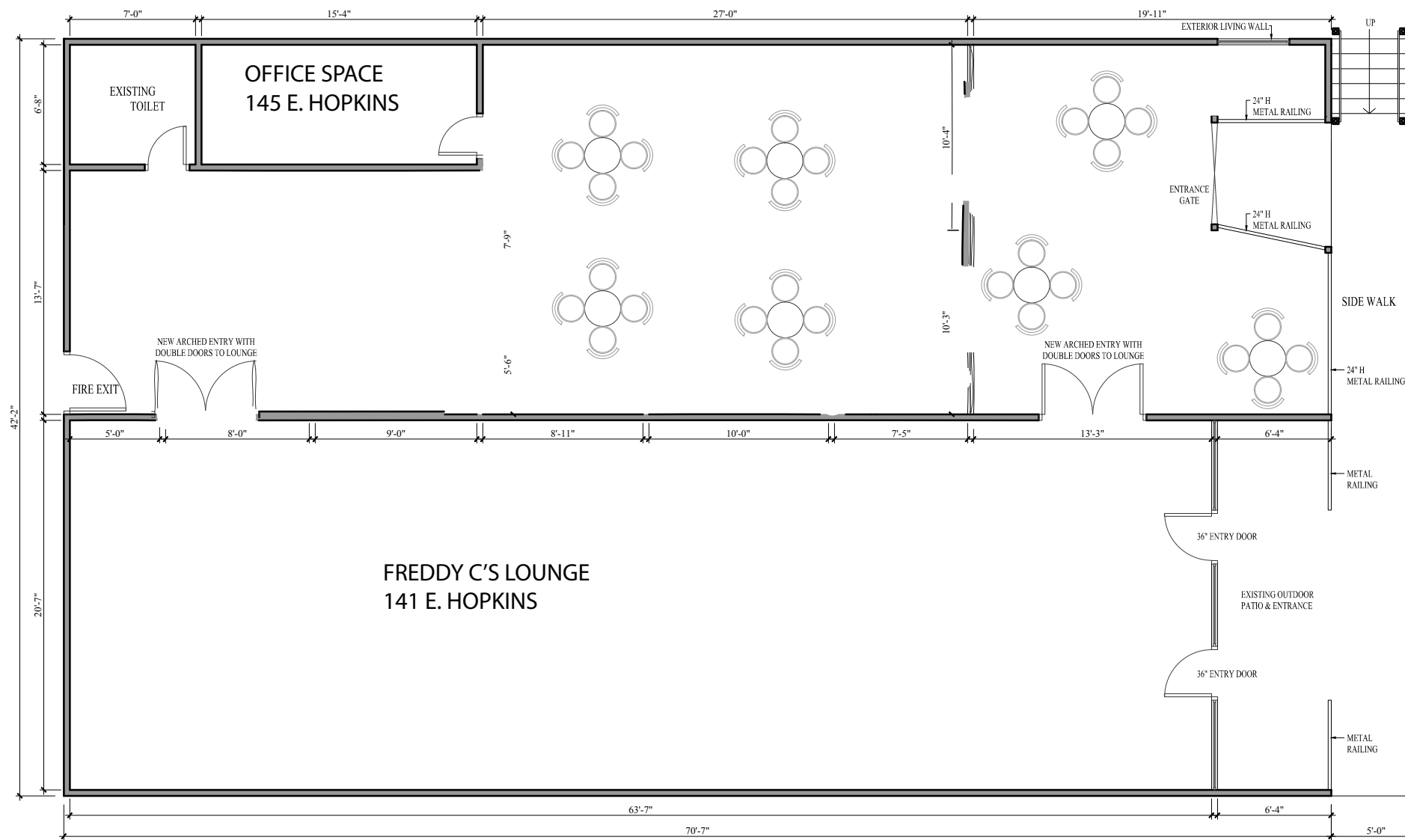
1 NEW- FIRST FLOOR PLAN SCALE : 1/8" = 1'-0"
