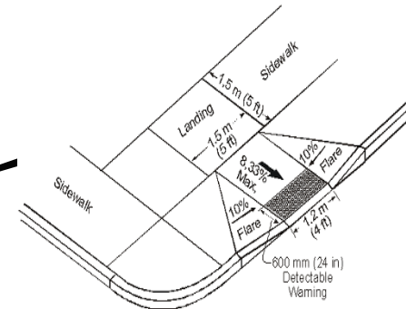
ADA Compliant Sidewalk Ramp For Mobility Disabilities
