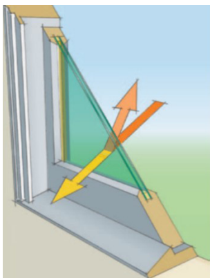
Windows with Low-E coating reflect back part of the summer sun. IMAGE SOURCE: Energy Savers, U.S. Department of Energy.
