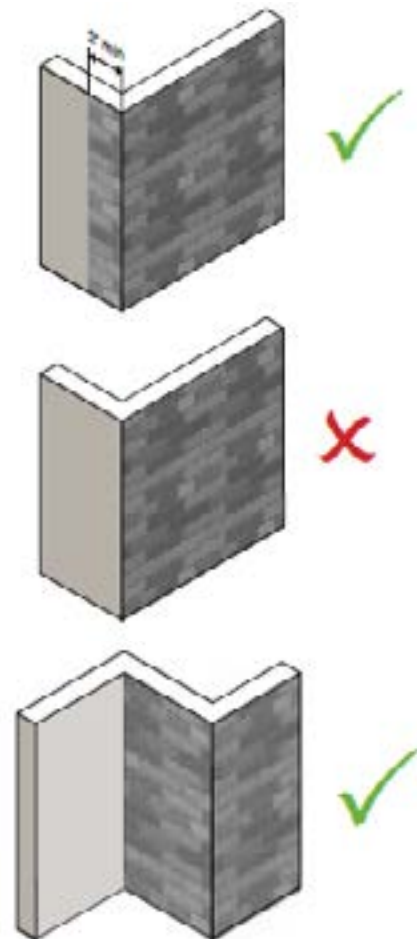
FIGURE 4.20 PRIMARY MATERIAL CHANGES
