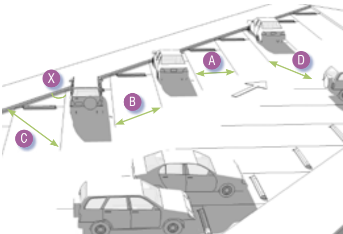
FIGURE 7.7 PARKING SPACE AND PARKING AISLE DIMENSIONS
