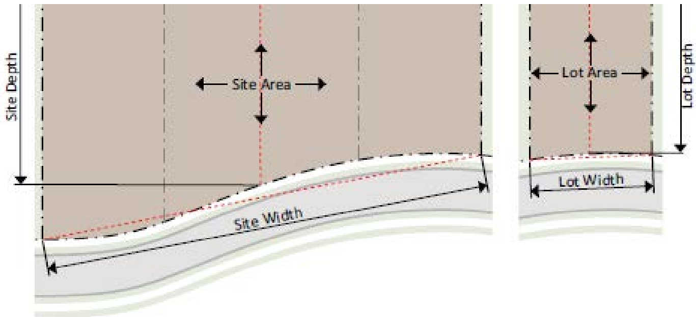
FIGURE 4.3 MEASURING SITES AND LOTS
