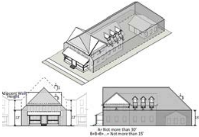
FIGURE 4.30 SETBACK PLANES
