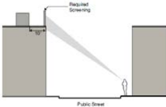
FIGURE 7.18 ROOF MOUNTED UTILITY SCREENING
