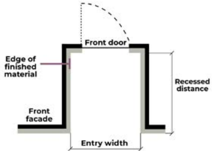
FIGURE 4.17 RESIDENTIAL FRONT DOOR REQUIREMENTS
