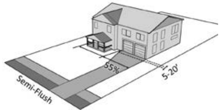
FIGURE 7.2 SEMI-FLUSH GARAGE
