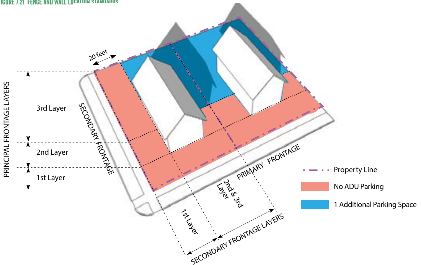
FIGURE 7.21 FENCE AND WALL LOCATION STANDARDS
