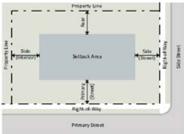
FIGURE 4.5 BUILDING SETBACKS
