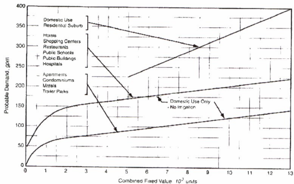
Figure 4-3 Water flow demand per fixture value—high range
