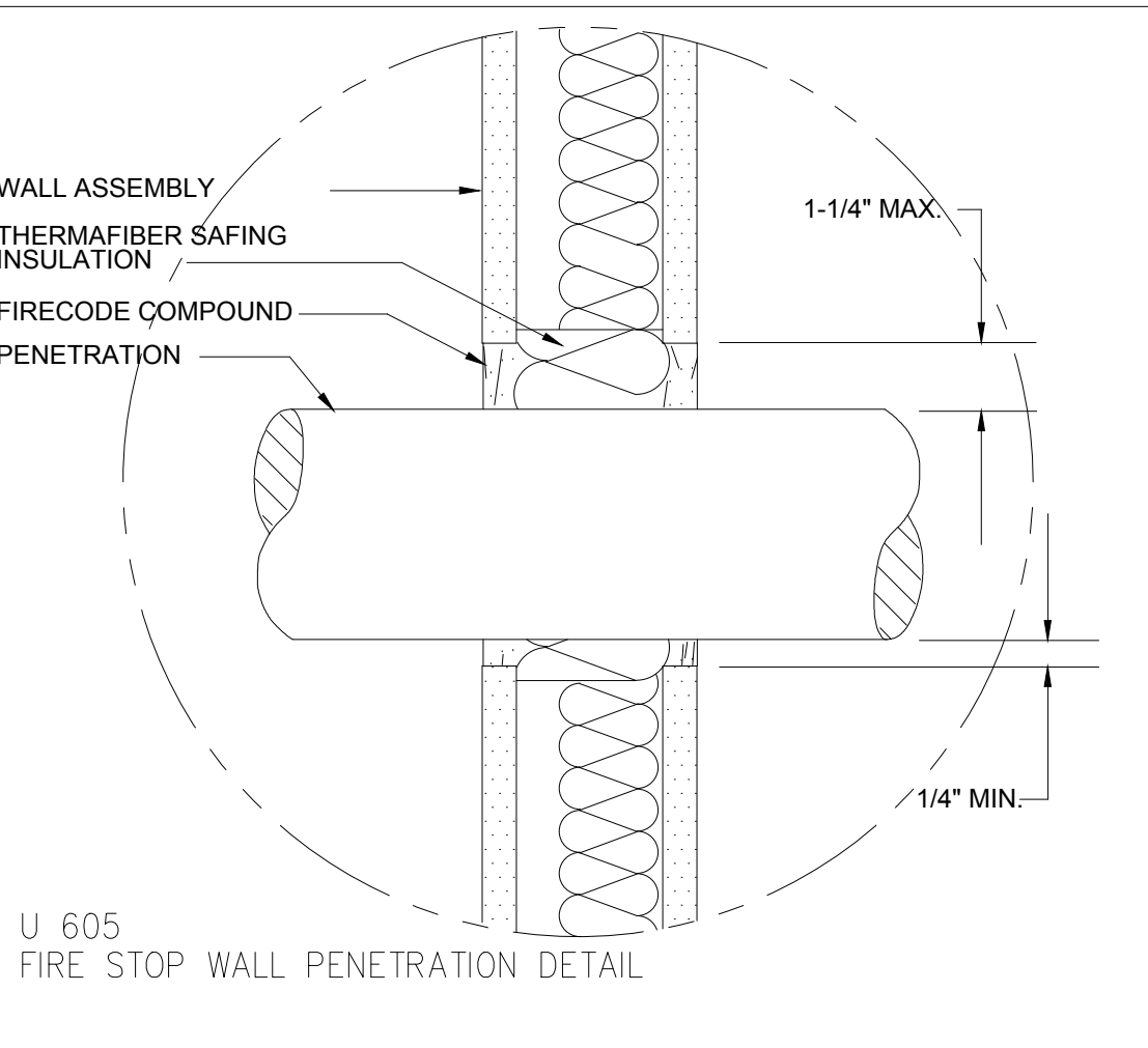
FIRE STOP WALL PENETRATION DETAIL 03
