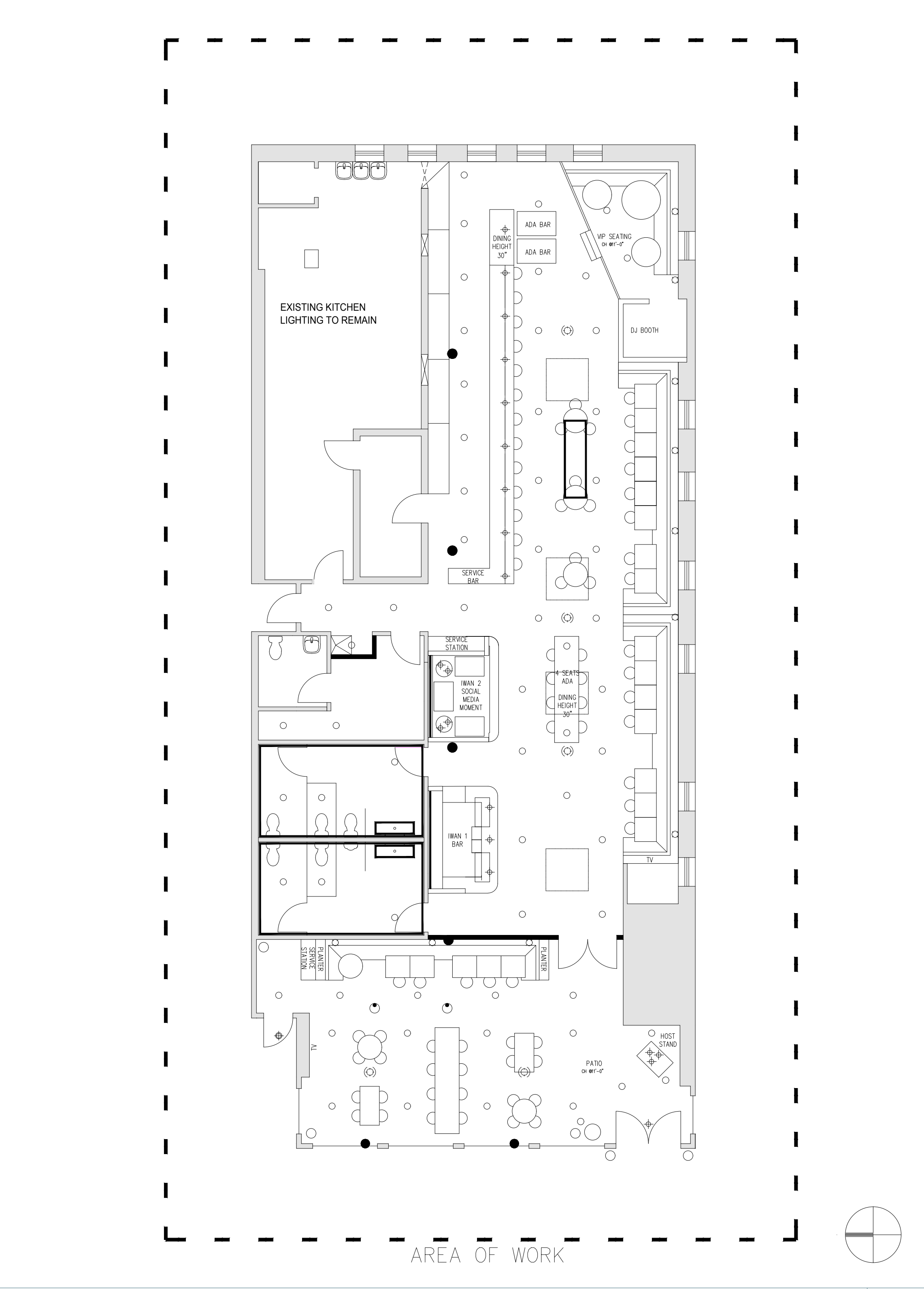
REFLECTED CEILING PLAN 04
