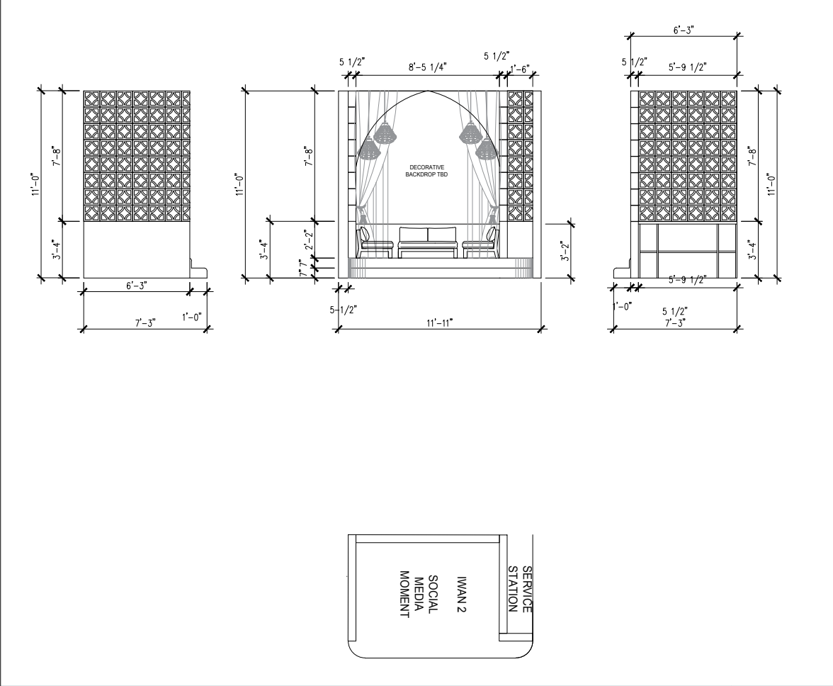
IWAN2 1/8" = 1'-0" 07
