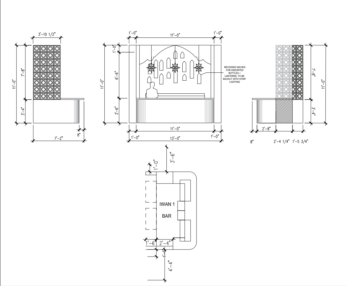
IWAN1 1/8" = 1'-0" 08
