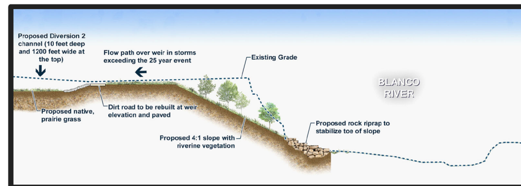
VEGETATED STABILIZATION
