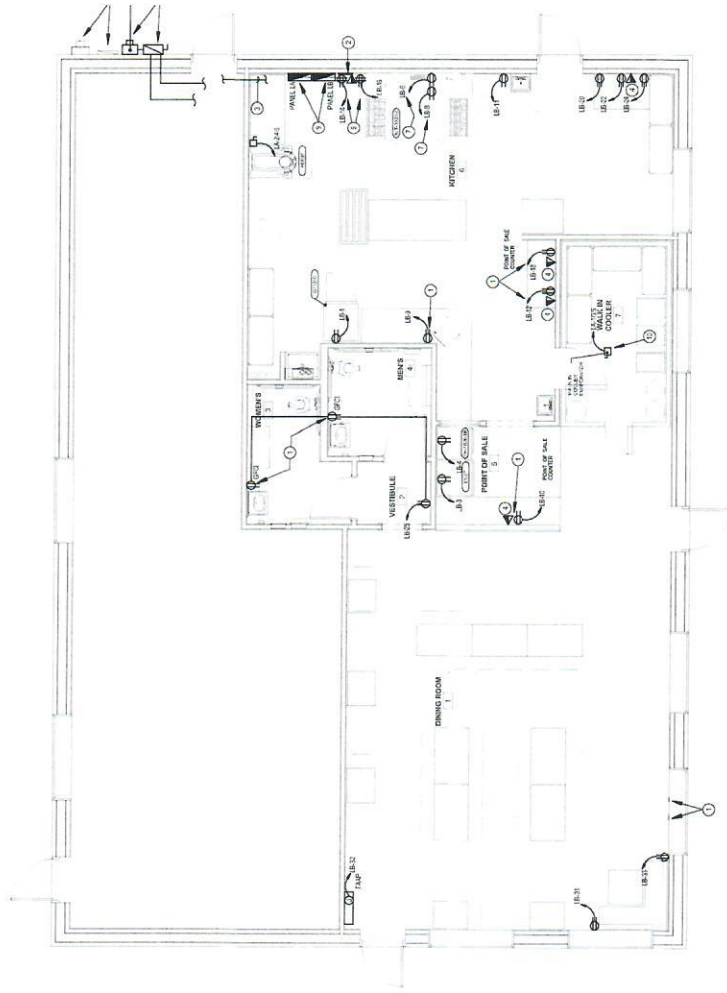
01 FIRST FLOOR PLAN - POWER SCALE: 1/4"=1'-0"
