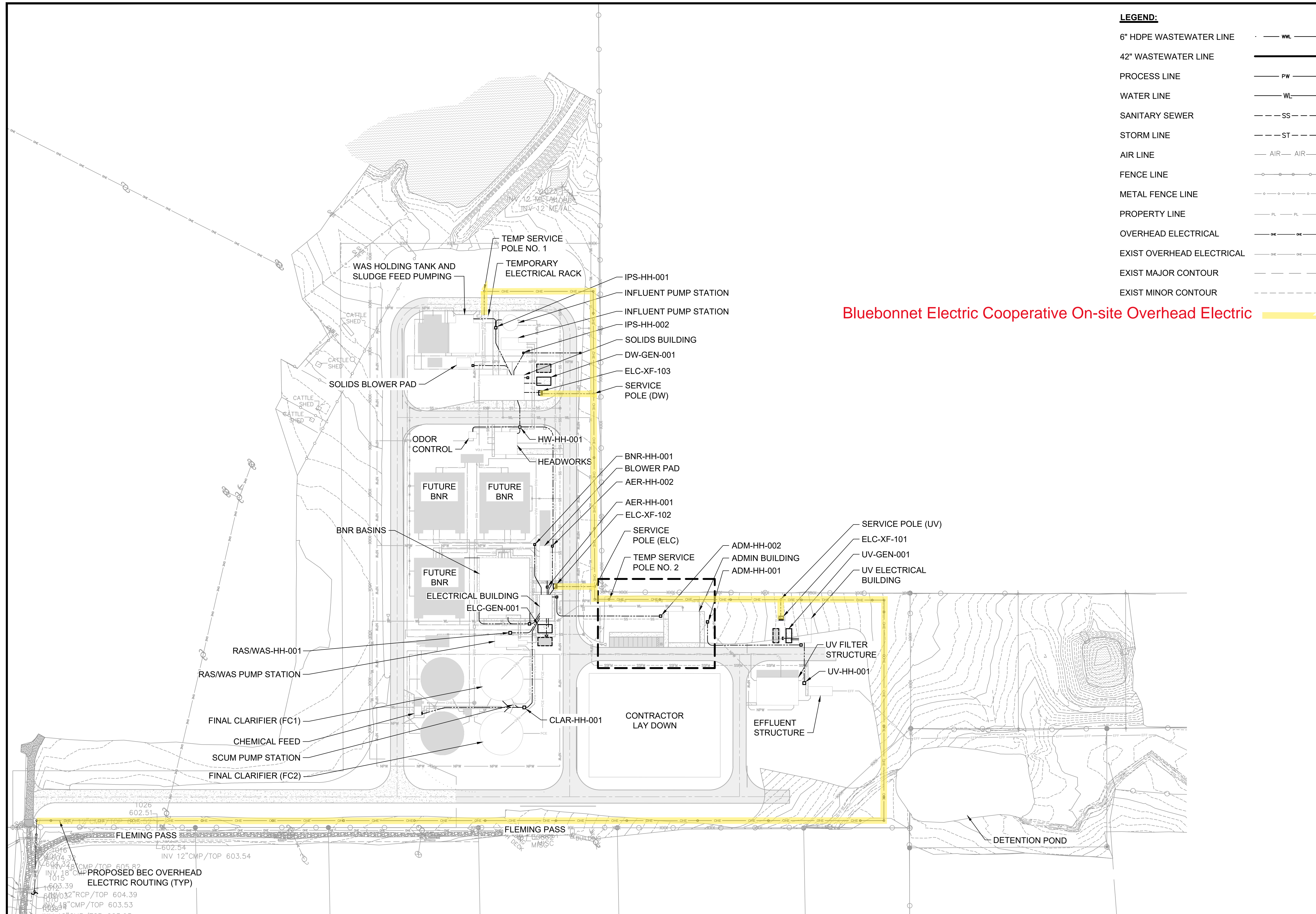
ELECTRICAL SITE PLAN 0 100' 200' HORIZONTAL SCALE IN FEET NORTH
