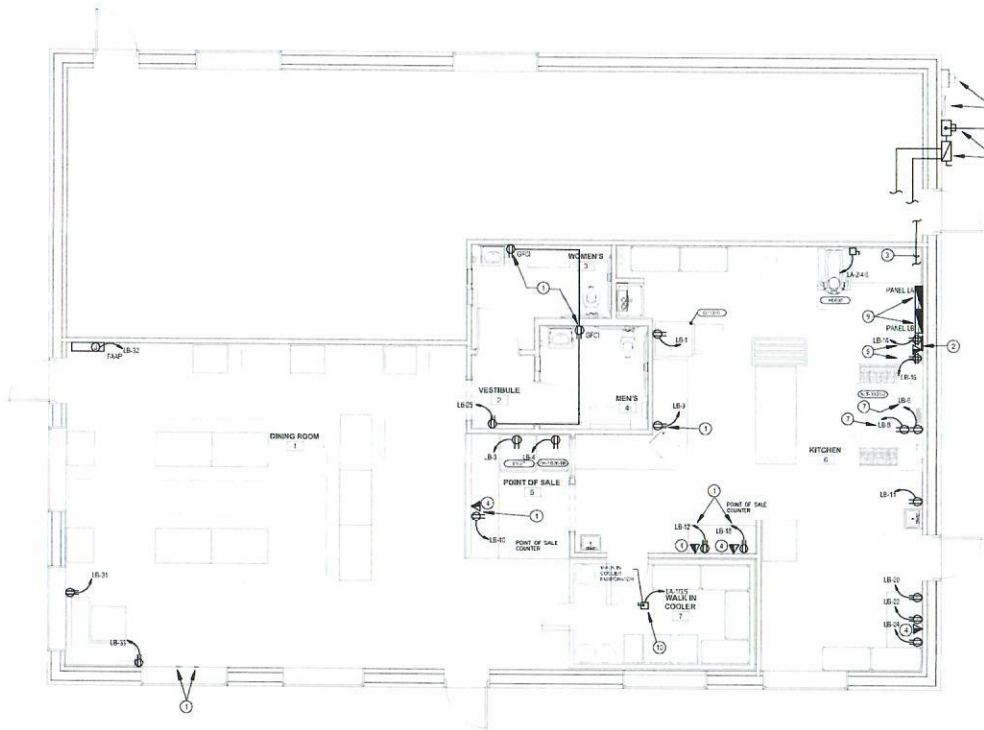
01 FIRST FLOOR PLAN - POWER SCALE: 1/4"=1'-0"
