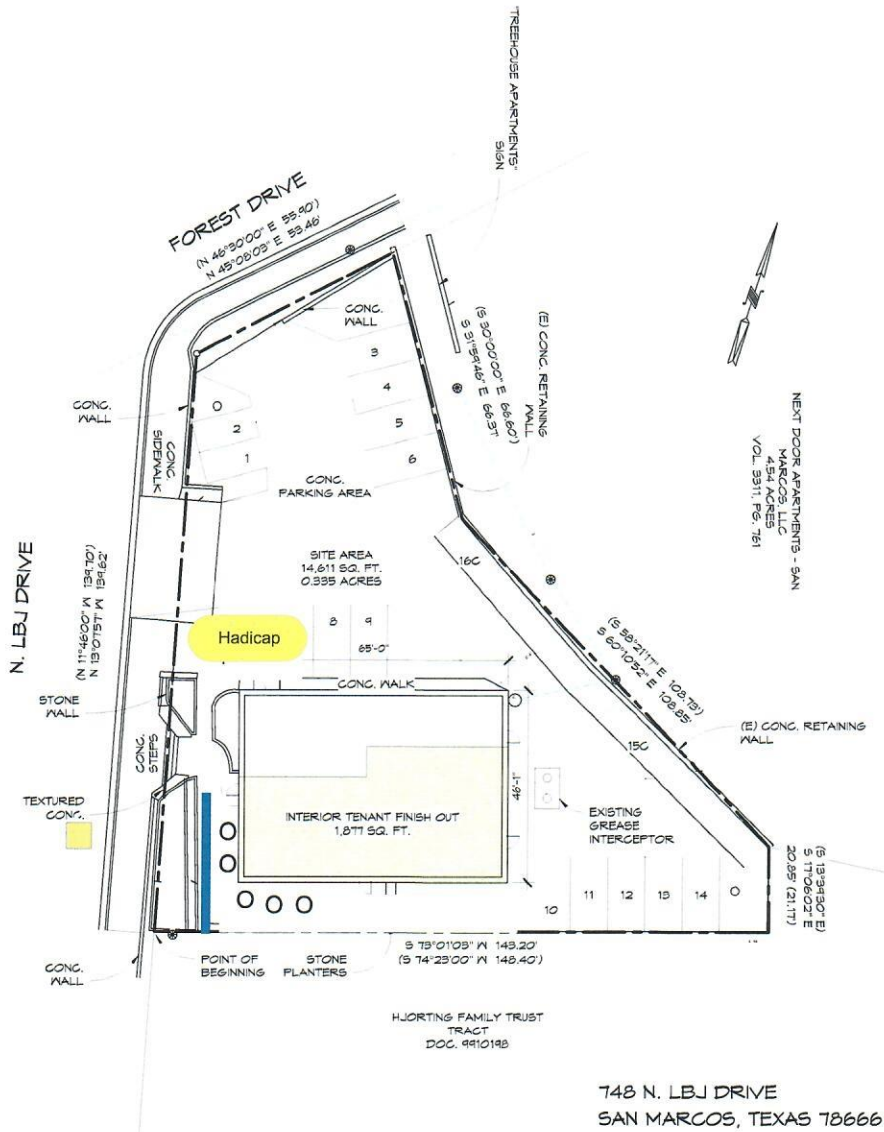
1 Site Plan 1" = 20'-0"
