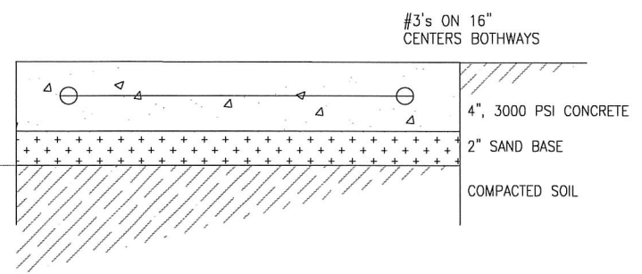
CONCRETE CROSS SECTION DETAIL
